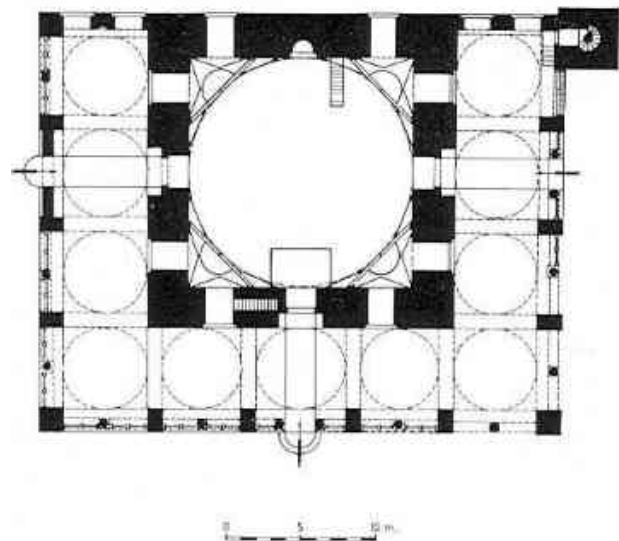
Fig. 33. The mosque of Sinān Pasha (Department of Antiquities).
